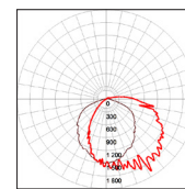
40W-4000K-110°
