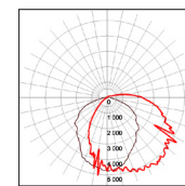
120W-4000K-110°
