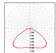
200W-5000K-120°
