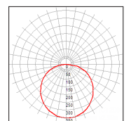
2X2 40W-4000K-113°
