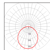
2X2 20W-4000K-113°
