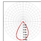
100W-5000K-60°
