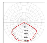
60W-5000K-120°
