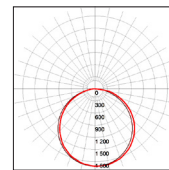
2X4 50W-5000K-110°
