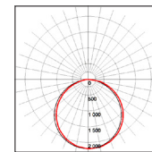
2X4 60W-5000K-110°
