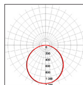
1X4 40W-5000K-110°
