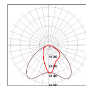
600W-5000K-65x120°
