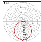
40W-3000K-110°
