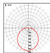
18W-3000K-110°
